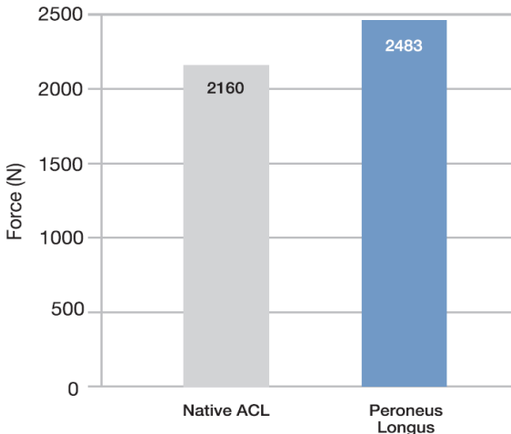
ULTIMATE LOAD FAILURE TEST 1
